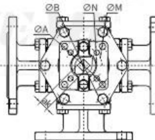
3-Way L-Port
